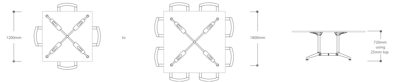
suits tables from 1200mm square minimum to 1800mm square maximum
