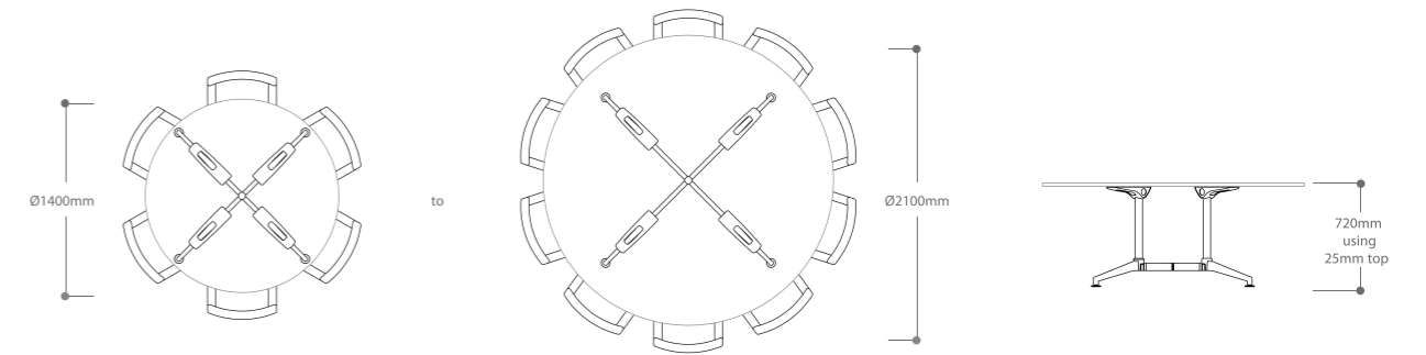
suits tables from 1400mm Ø minimum to 2100mm Ø maximum
