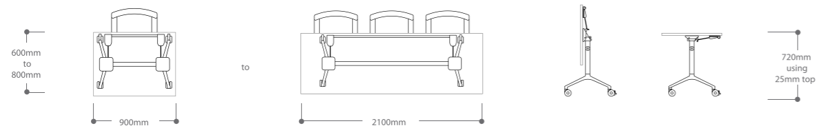
available in four beam lengths to suit tables from 900mm minimum to 2100mm maximum
