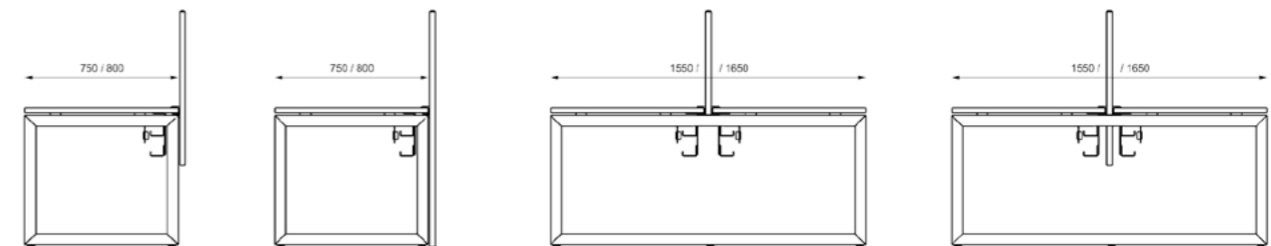
CABLE MANAGEMENT - SCREEN ORIENTATION
