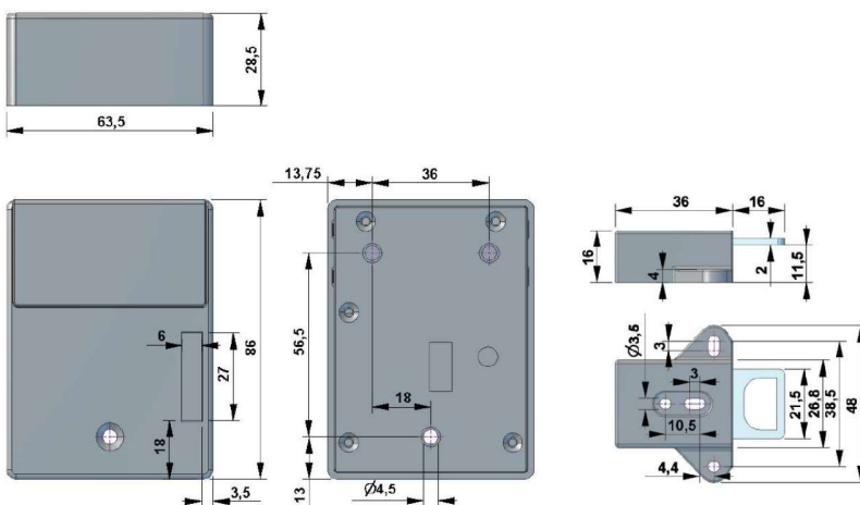
Technical specifications of the latch lock PROXY RFID125 kHz
