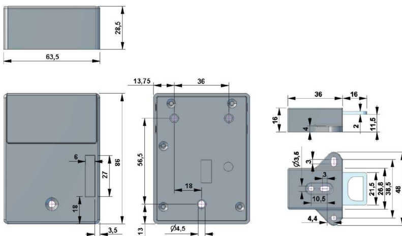
Technical specifications of the Locker lock
