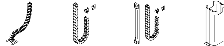
Cable chain with floor infeed
