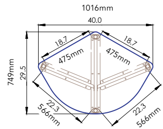
Model SS03002 Bottom View
