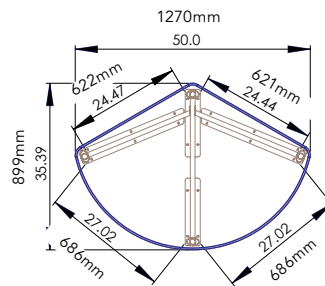
Model SS03011 Bottom View
