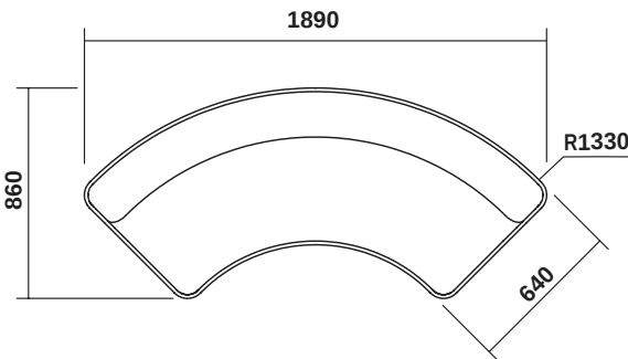
CIR-M-2030-LB/HB WITH LOW - OR - HIGH PRIVACY SCREEN
